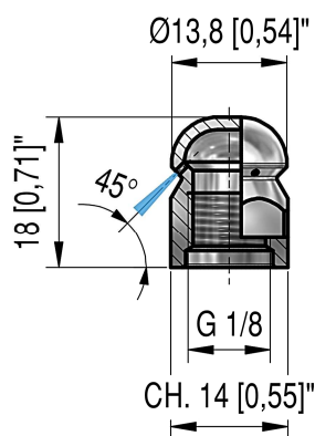
ST3 STURATUBO FISSI - 3 FORI ST3 DRAIN CLEANING NOZZLE - 3 HOLES
